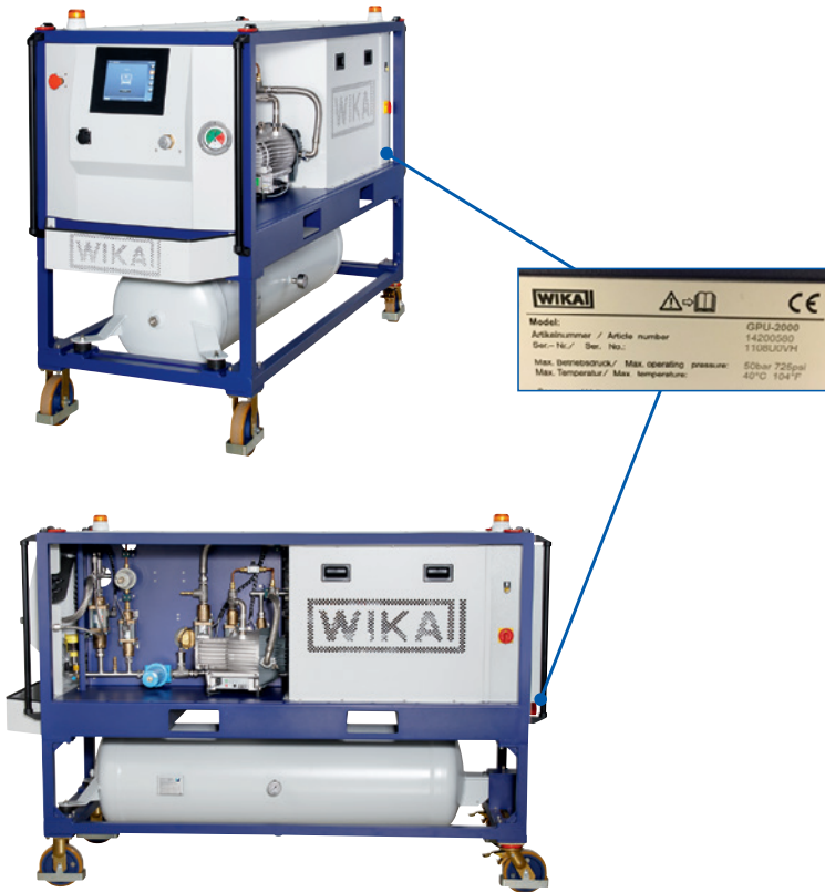
Handling equipment for SF 6 gas
